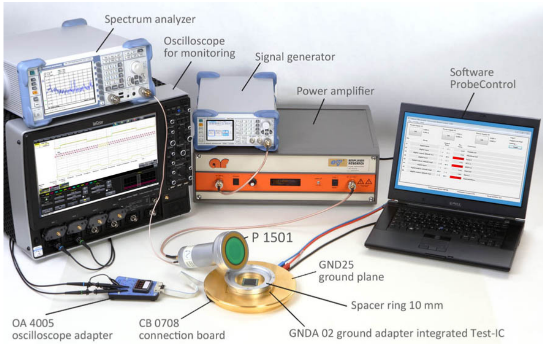
Measurement set-up with P1501 RF E-Field source
