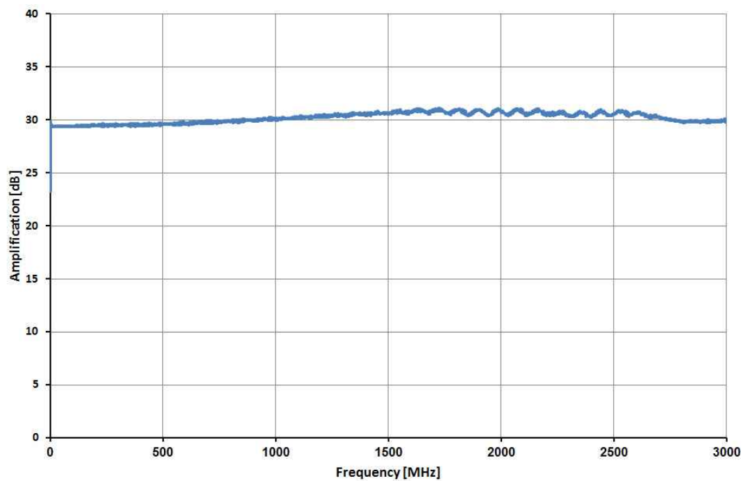
Frequency response
