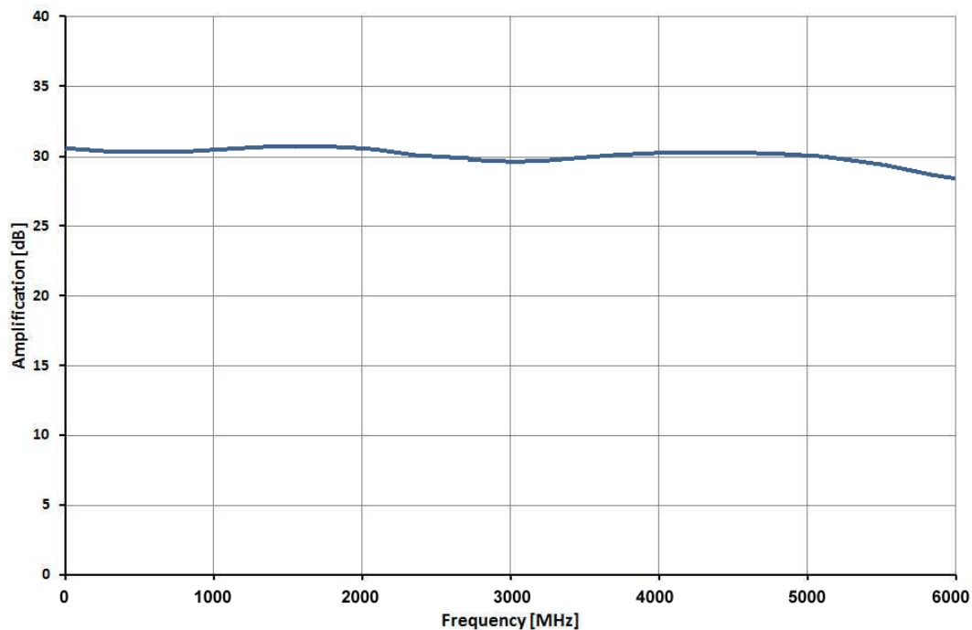
Frequency response
