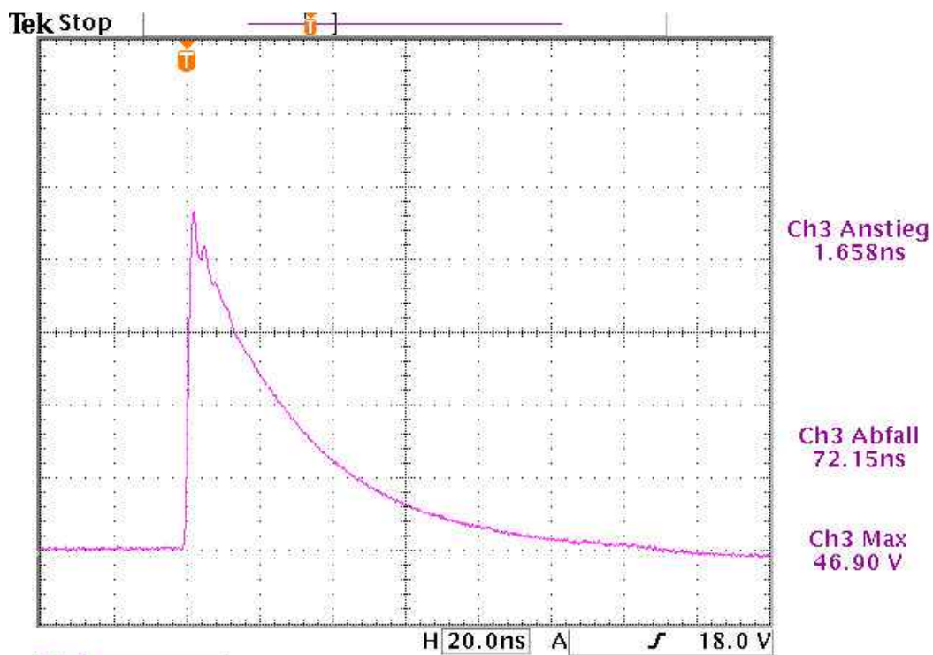
Pulsform (gemessen)
