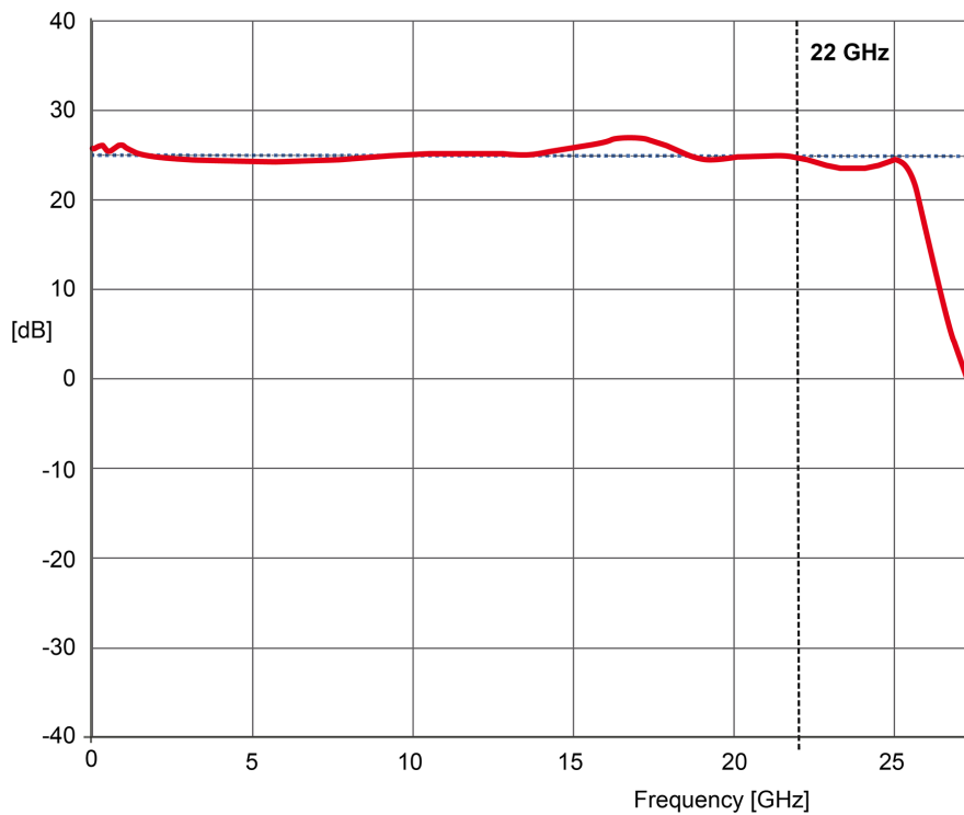
Frequenzgang
