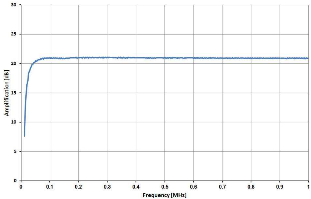
Frequenzgang (Detail)
