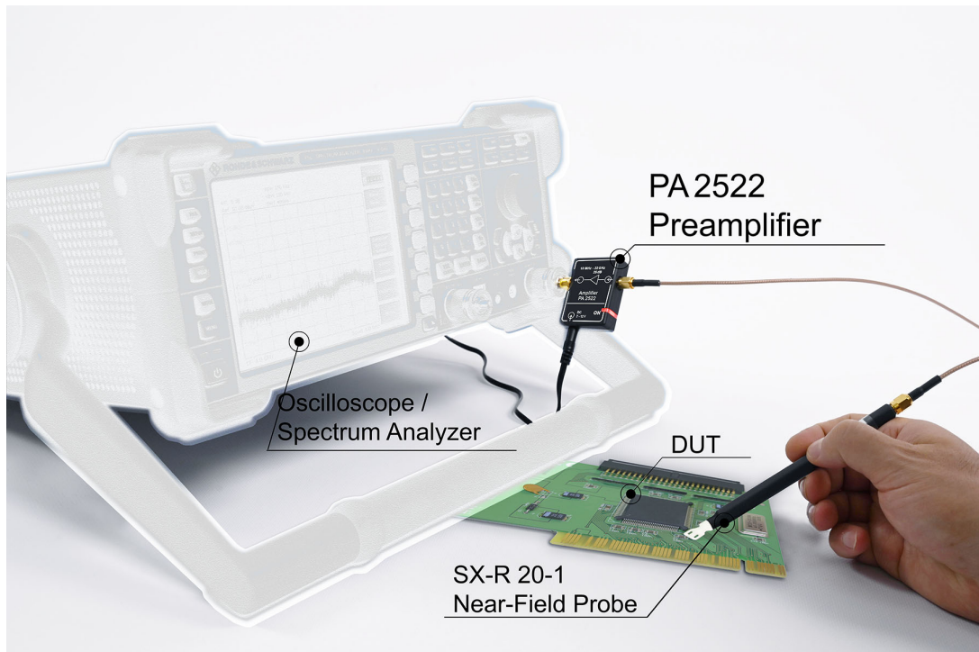
Measurement set-up with PA 2522
