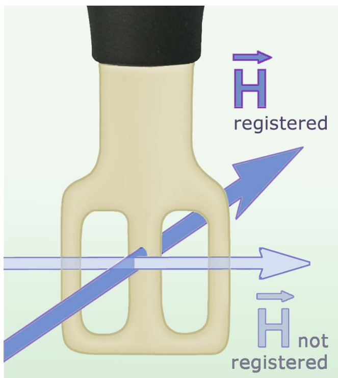
SX-R 20-1 probe head
